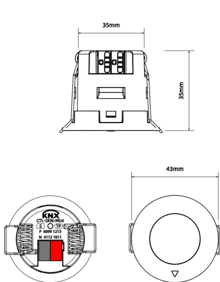
Figure 1 Dimension Diagram
