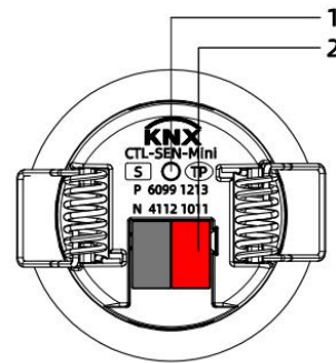
Figure 2 Component Diagram
