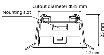
Cutout diameter Ø35 mm
