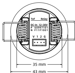
Front diameter Ø43 mm
